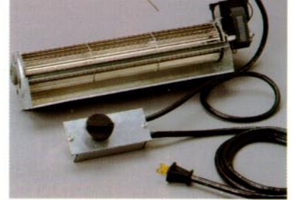
The optional GA3700 blower accessory can be installed in any circulating louvered LogMate Firebox or the stove to maximize heat distribution. Features a variable speed control.
