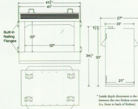
Side View for Both 36" and 42" Models
